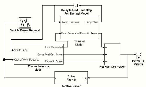
Fig.1: Block Diagram of the Fuel Cell Model
